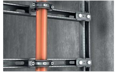
Vertical installation
