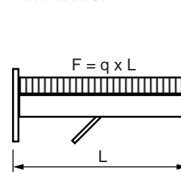
Load case 3a
