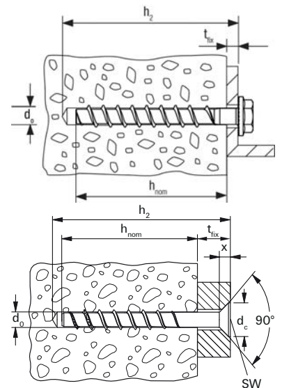
Concrete screw FBS-US A4 with hexagon head and molded washer, stainless steel A4
