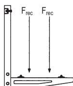
Load case 2
