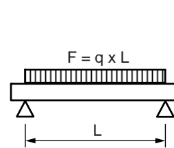
Load case 3
