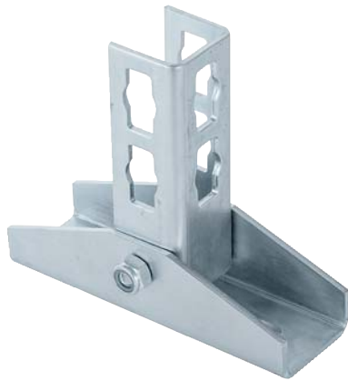
Massiv bracing of cantilever arm
